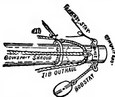
RIG OF RUNNING BOWSPRIT.
